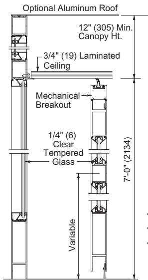
Vertical Section
