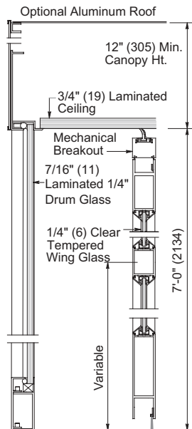
Vertical Section
