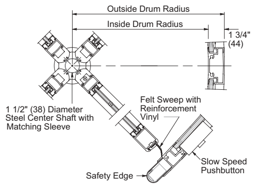
Horizontal Section
